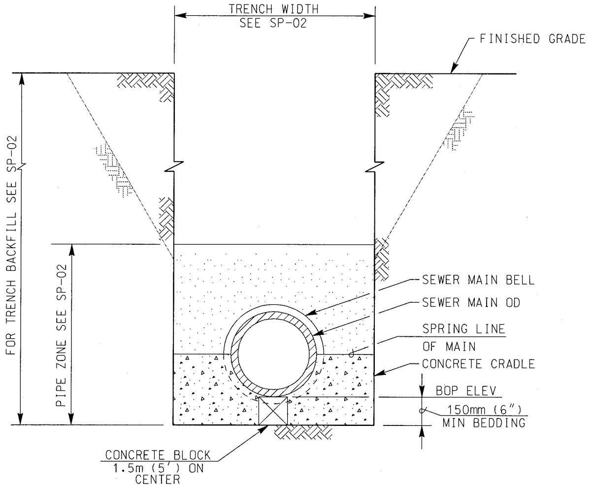
TRENCH SECTION
